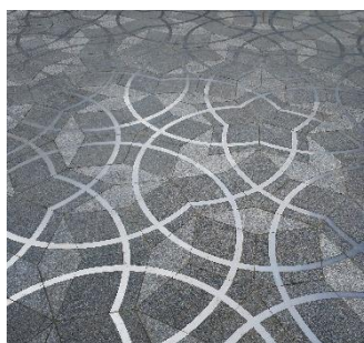
↑ Penrose tiling
